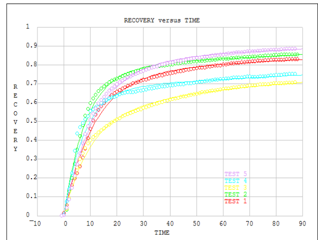
Figure 3: Plot of metal recovery curves versus time achieved through testwork and curve-fit in METSIM.
