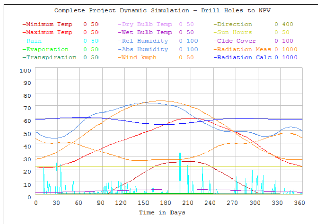
Figure 4: Plot of site weather data over a one year span, including temperatures, rainfall, evaporation, cloud cover, wind, and humidity.
