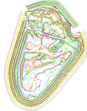
Figure 5: Tailings dam contours used to generate a block model of the waste facility.
